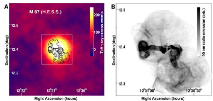
Fig. 3: The radio galaxy M 87 seen at very high energies by H.E.S.S. (left panel (A), colour scale). The emission seems extended which is, however, explained by the
