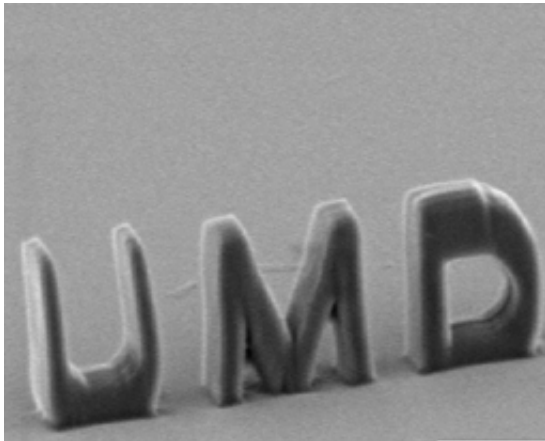
These microscopic University of Maryland letters were made with the PDMS wall method. The wall has been removed from the M and D. Credit: The Fourkas group.
