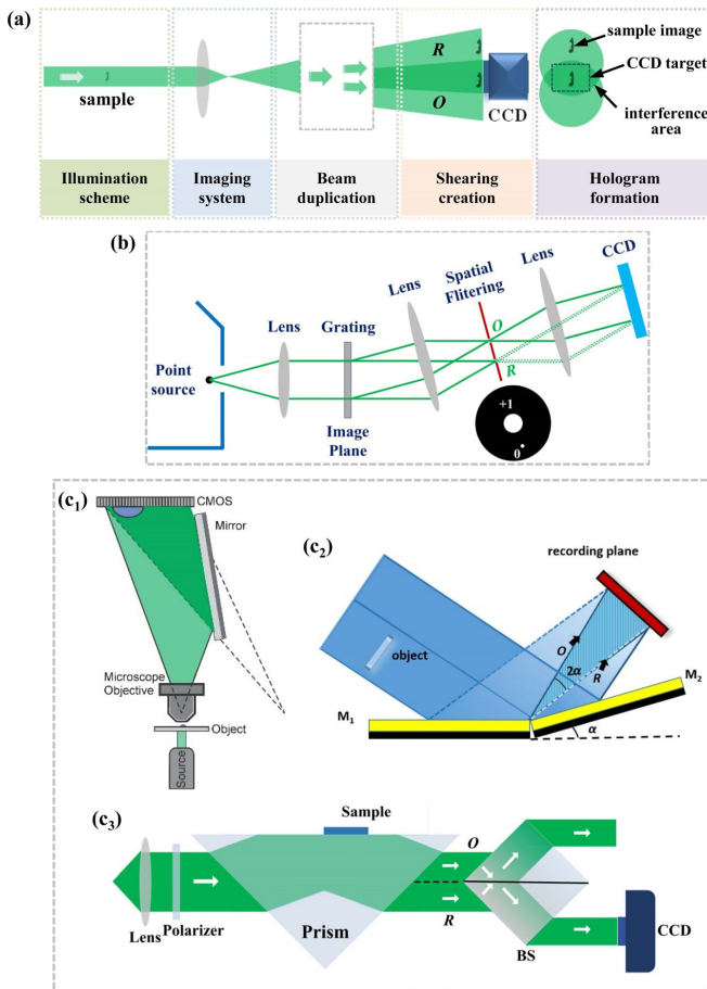
(a), (b) Concepts of common-path configuration based on lateral shearing and point diffraction. (c 1 -c 3 ) Experimental setups of common-path digital holography using folding Lloyd's mirror, mirror pair, and specially-positioned beam splitter cube. Credit: Jiwei Zhang, Siqing Dai, Chaojie Ma, Teli Xi, Jianglei Di, and Jianlin Zhao
