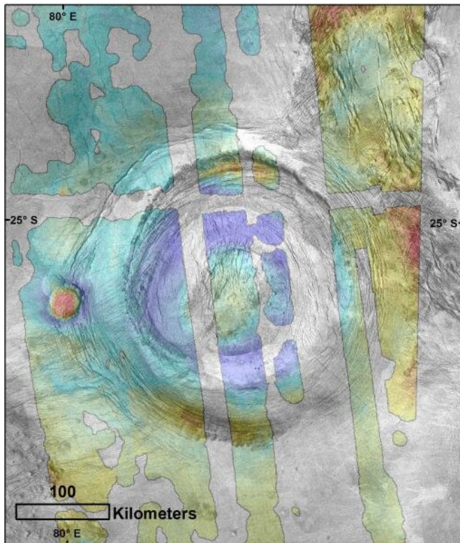
Magellan SAR image of Aramaiti Corona. Narina Tholus (center left) appears as two adjacent domes that are superposed on the west outer fracture ring. Credit: Planetary Science Institute
