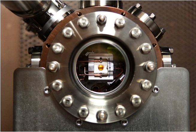
The centerpiece of the quantum computer: the ion trap in a vacuum chamber. Credit: University of Innsbruck
