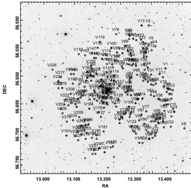
The observed image in V band which contains open cluster NGC 281. The stars detected as variables are encircled. Credit: Lata et al., 2021.
