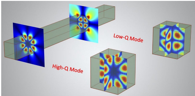
High-Q and low-Q Mie modes of single dielectric 2D nanowire (left) and finite 3D nanoparticle (right). Credit: L. Huang et al.
