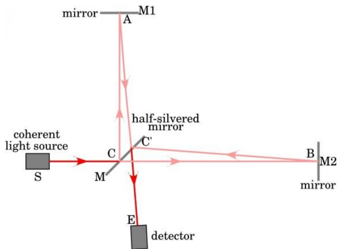
How to measure the round-trip speed of light. Credit: Wikipedia user Krishnavedala
