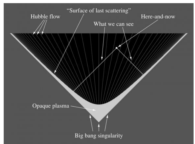
A Milne universe with anisotropic light would look uniform. Credit: Wikipedia user BenRG
