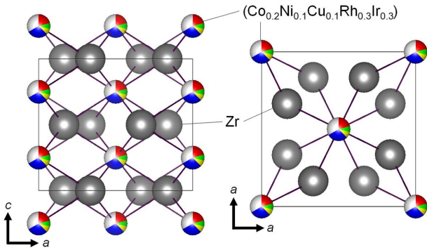
Schematic of the \text{CuAl}_2 -type crystal structure of the newly created superconducting \text{Co}_{0.2}\text{Ni}_{0.1}\text{Cu}_{0.1}\text{Rh}_{0.3}\text{Ir}_{0.3}\text{Zr}_2 compound, with an HEA-type Tr site. Credit: Tokyo Metropolitan University
