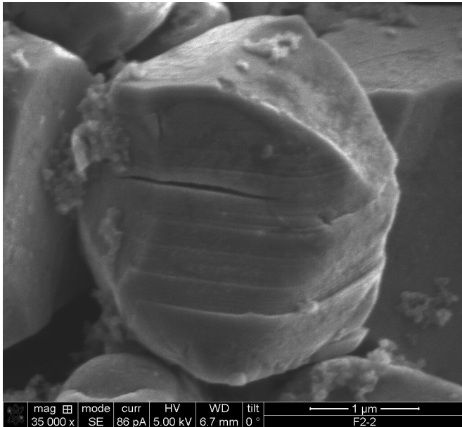
A nickel-rich single crystal created by the PNNL team. Credit: PNNL
