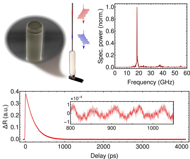
Top-left : SEM image of the micropillar optophononic resonator, and fibered device. Top-right: Acoustic spectrum of the nanomechanical resonator. Bottom: time trace measured using a fibered pump-probe coherent phonon generation scheme. Credit: Centre for Nanoscience and Nanotechnology
