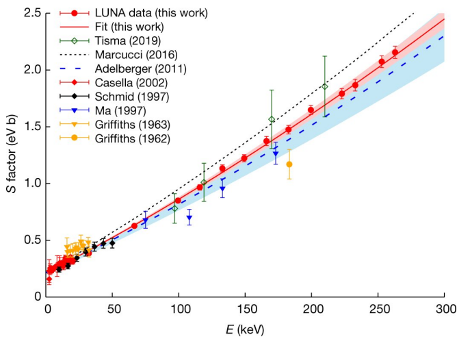
The S factor of the D(p,?)^3\text{He} reaction. Credit: Nature (2020). DOI: 10.1038/s41586-020-2878-4
