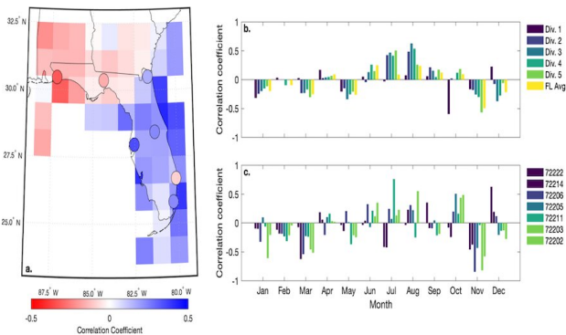
(a) Map of the correlation between Atlantic SSTs and precipitation for June - October in GPCP (squares) and rain gauges (circles). (b and c) correlation between Atlantic SSTs and precipitation by month in nClimDiv (b) and rain gauges (c). Credit: Jeremy Klavans
