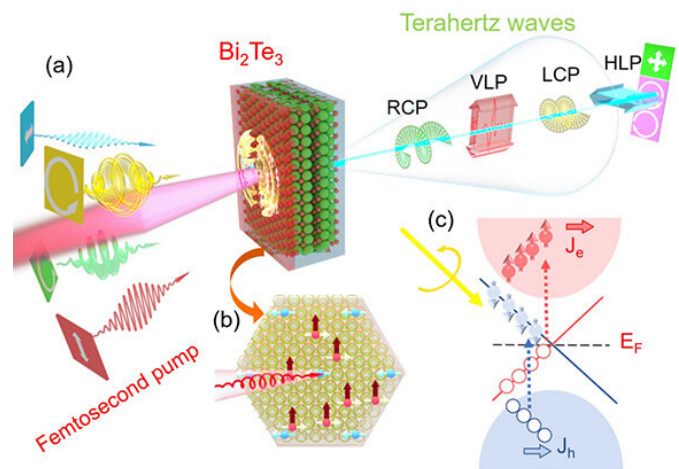
Schematic diagram of the polarization tunable THz emission from \text{Bi}_2\text{Te}_3 . (a) Femtosecond laser pulses with horizontal linearly polarized (HLP), vertical linearly polarized (VLP), left-handed circularly polarized (LCP), and right-handed circularly polarized (RCP) illuminate onto the topological insulator \text{Bi}_2\text{Te}_3 and produce polarization tunable THz waves. (b) Macroscopic helicity-dependent photocurrents and only unidirectional spin current can be generated. (c) Microscopic electronic transition under circularly polarized laser pulse illumination. Credit: SPIE
