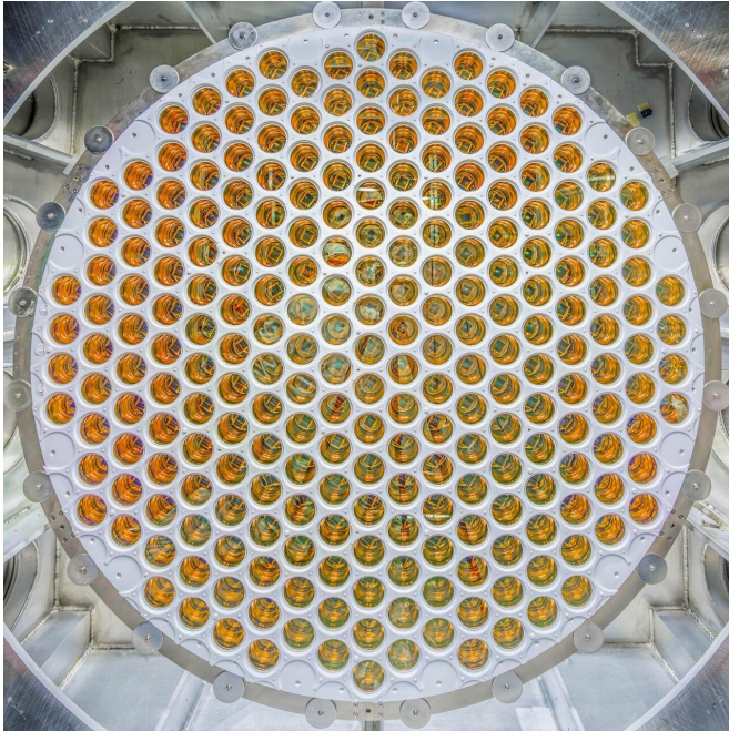
This array of photomultiplier tubes is designed to detect signals occurring within LZ's liquid xenon tank. Credit: Matt Kapust/Sanford Lab
