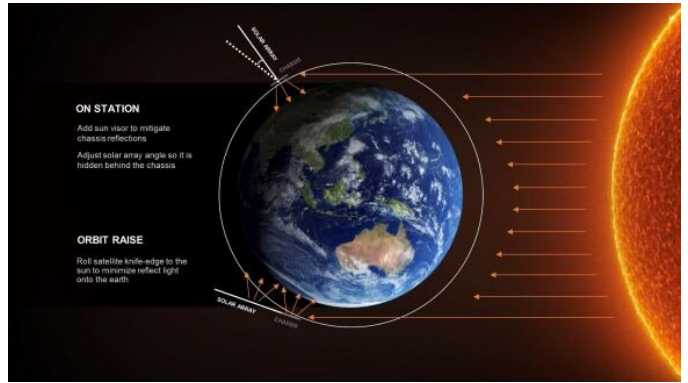
Illustration of Starlink orbits and their reflective qualities. Credit: SpaceX
