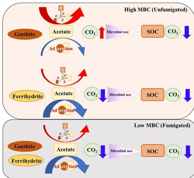
Conceptual model of the effect of iron oxides on CO 2 emissions in anaerobic paddy soil with different levels of MBC. Credit: LI Yuhong
