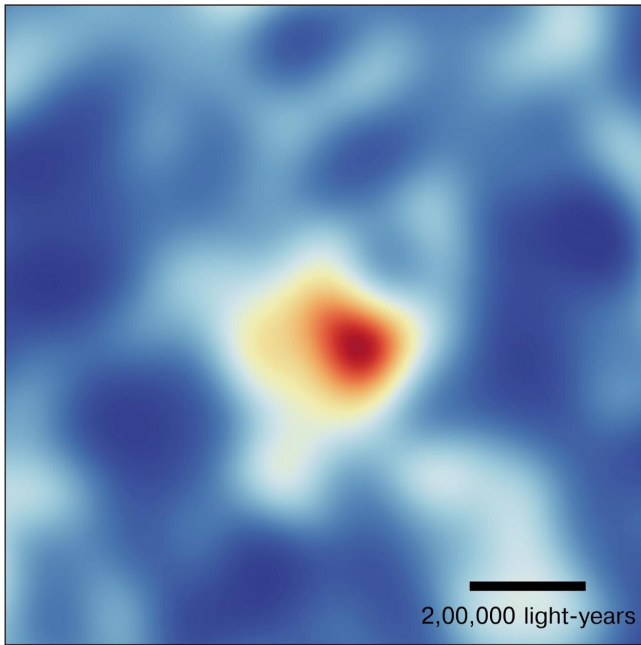
An image of the stacked 21 cm signal detected with the upgraded GMRT, arising from atomic hydrogen gas in galaxies 22 billion light years away. Credit: Chowdhury et al.
