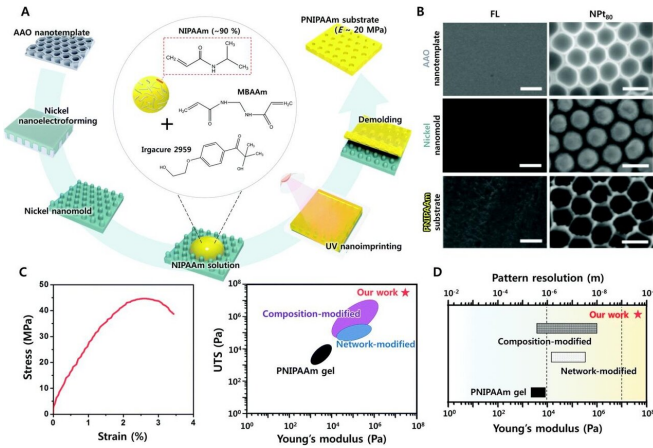
Design of the bulk PNIPAAm nanopore-patterned surface. (A) Diagram showing the three-step nanoreplication process consisting of aluminum anodizing, nickel nanoelectroforming, and UV nanoimprinting. (B) SEM images (scale bar: 500 nm) of PNIPAAm FL and NPt80 created in each step of the nanoreplication process. (C) The mechanical characterization; and (D) replicable pattern resolution of the PNIPAAm NPt substrates compared to various PNIPAAm hydrogels in different forms. Credit: POSTECH
