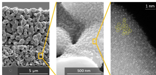
(left) solid oxide fuel cell electrode(center) a single atom
