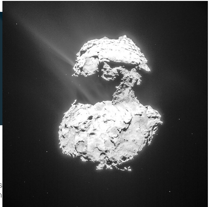
Gas and dust rise from Chury's surface as the comet approaches the point of its orbit closest to the Sun. Credit: ESA/Rosetta/NAVCAM
