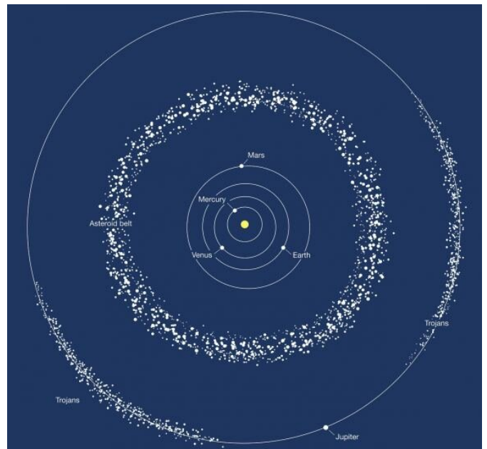
This image depicts the two areas where most of the asteroids in the Solar System are found: the asteroid belt between Mars and Jupiter, and the trojans, two groups of asteroids moving ahead of and following Jupiter in its
