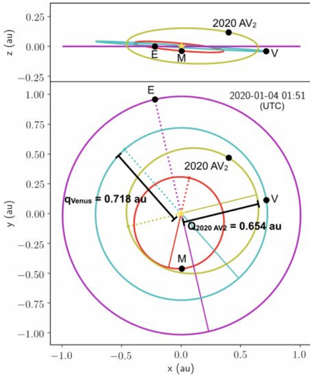
This image from the study shows 2020 AV2's orbit. It also shows the orbits of Earth, Mercury and Venus. Perihelions are dotted lines, and aphelions are solid lines. Credit: Ip et al, 2020
