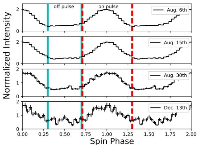
X-ray folded light curves of PSR J1119?6127 in the 0.5–10.0 keV energy band from XMM-Newton. Credit: Wang et al., 2020.
