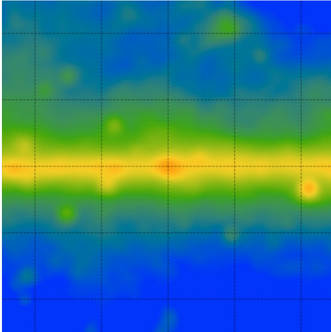
This representation of data from the Fermi Gamma Ray Space Telescope after its launch in 2008 shows an excess of high-energy radiation in the Milky Way's Galactic Center. Many physicists attributed this to the annihilation of weakly interacting dark matter particles, but a UCI-led study has excluded this possibility through a range of particle masses. Credit: Oscar Macias for UCI
