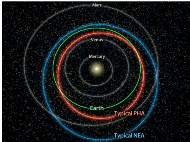
Image showing the eccentricities of the innermost planets and asteroids. Credit: NASA / JPL-Caltech
