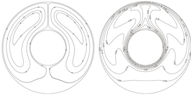
Simulation results of natural convection in a concentric annulus at Ra=5 \times 10^4 , streamlines (left), temperature contours (right). Credit: SIAT
