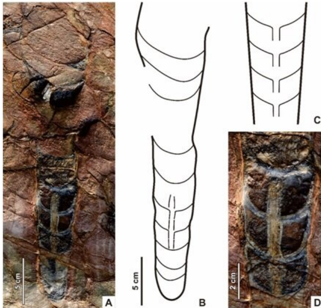
Sinoceras chinense , collected from Si Sawat county of Kanchanabura Province, western Thailand. Credit: NIGPAS
