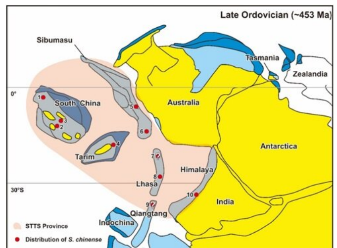
Distribution of S. chinense in the northeastern peri-Gondwana region. Credit: NIGPAS
