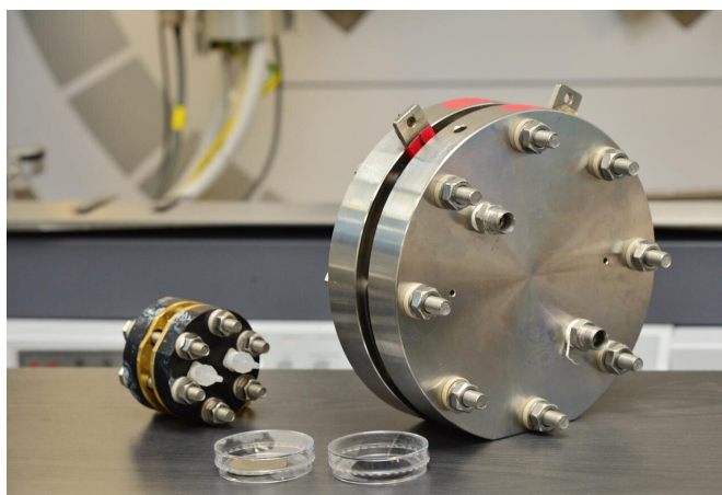
(Right) Coral shape silver nano-catalyst electrode with high-performance, large-area developed by KIST researchers (electrode size 50 cm) (Left) Catalyst electrode for synthetic photosynthesis in existing gas state (electrode size 2cm) Credit: Korea Institute of Science and Technology(KIST)
