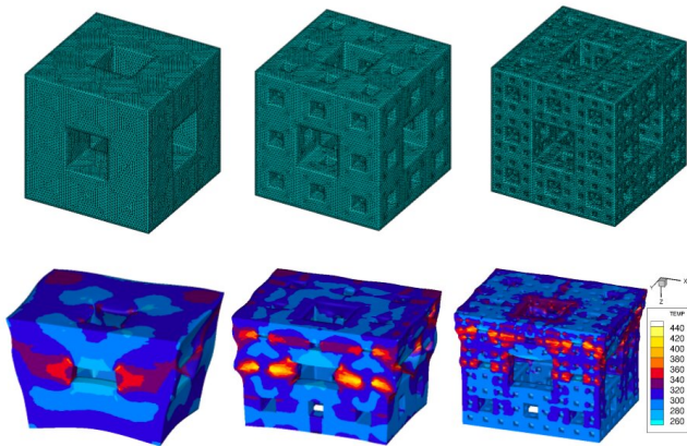
Simulations show how fractal structures of increasing complexity dissipate energy from shockwaves. Credit: Los Alamos National Laboratory
