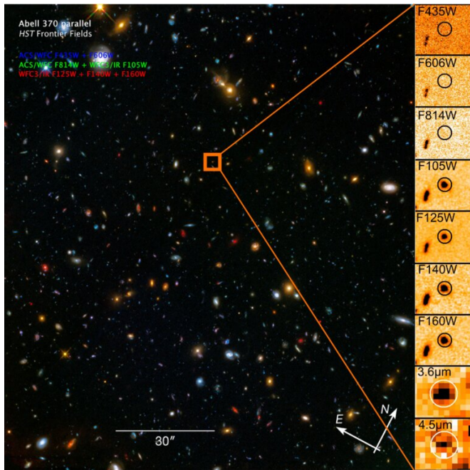
The galaxy A370p_z1 in the Hubble imaging and a zoom-in in each filter. The non-detection in the first three filters, followed by detections in all the redder filter is a typical signature of distant galaxies. Credit: NASA, ESA, Z. Levay (STScI)
