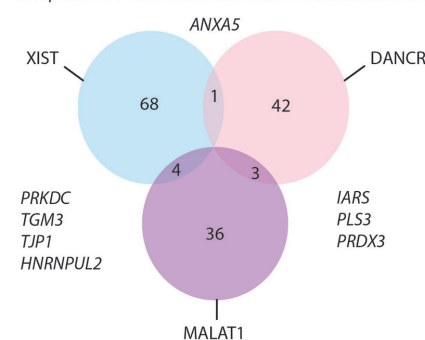
Comparison of CARPID Results Between Different lncRNAs
