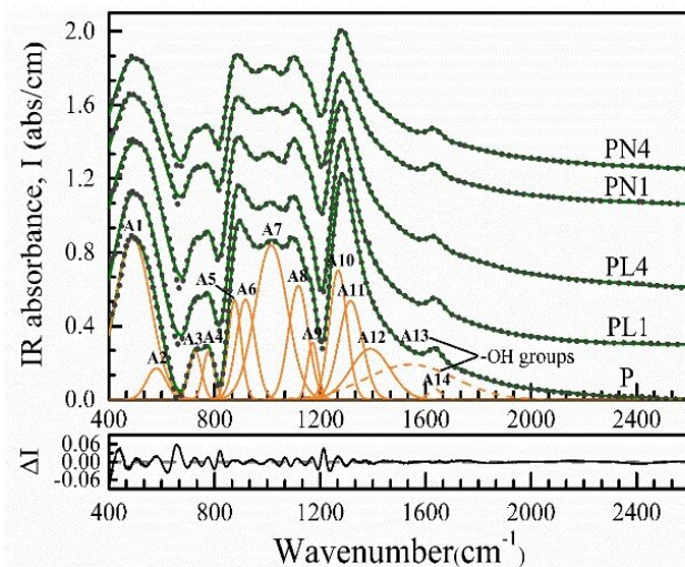
Measured and curve-fitting derived IR spectra of P, PL, PN glass samples, and individual bands of P glass according to literature. Credit: SIOM
