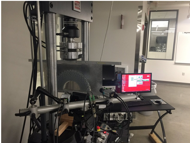
Lab equipment used to conduct experiments in the study. Credit: University of Missouri
