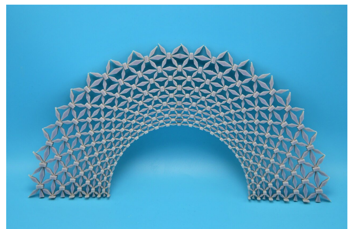
This structured lattice-type material protects against both types of energy waves -- longitudinal and shear -- that can travel through the ground. Credit: University of Missouri
