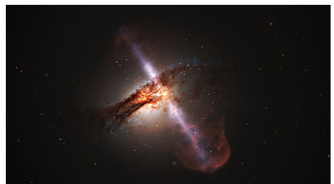
An active galactic nucleus, or quasar, hosts a black hole with an accretion disk of matter orbiting around and two jets of plasma beaming outward. Credit: ESA/Hubble, L. Calçada (ESO)
