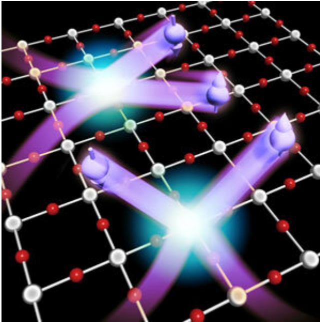
Figure 1: Electrons (lilac) interact strongly with one another as they move through the NiO 2 layer of a nickelate material, which could act as a model for high-temperature superconductivity (nickel = gray, oxygen = red). (Image produced by Mari Ishida of the RIKEN Center for Emergent Matter Science.). Credit: RIKEN Center for Emergent Matter Science
