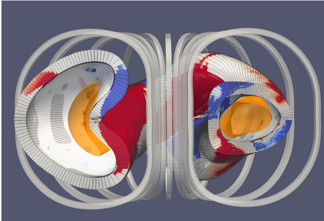
Schematic image of permanent magnet stellarator with plasma in yellow. Red and blue indicate permanent magnets with simplified coils surrounding the vessel. Credit: Coaxing Zhu.
