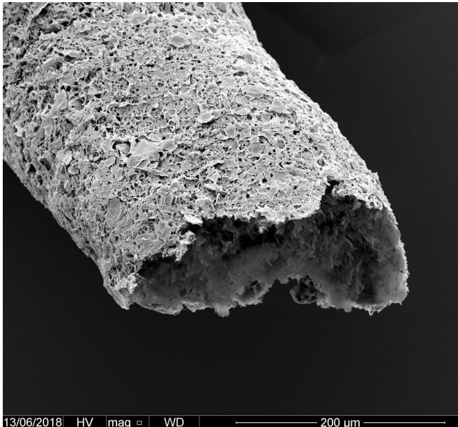
Close-up of a tubular structure made by simultaneous printing and self-assembling between graphene oxide and a protein. Credit: Professor Alvaro Mata
