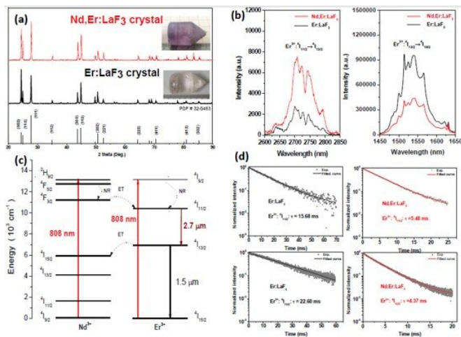
Characterization of Nd,Er:LaF 3 crystal. Credit: SIOM
