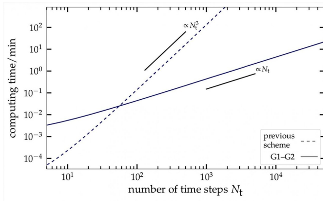
Computing time required for the new G1-G2 method (solid line) as a function of the process duration, compared to the traditional method (logarithmic scale). Credit: Niclas Schlünzen, AG Bonitz
