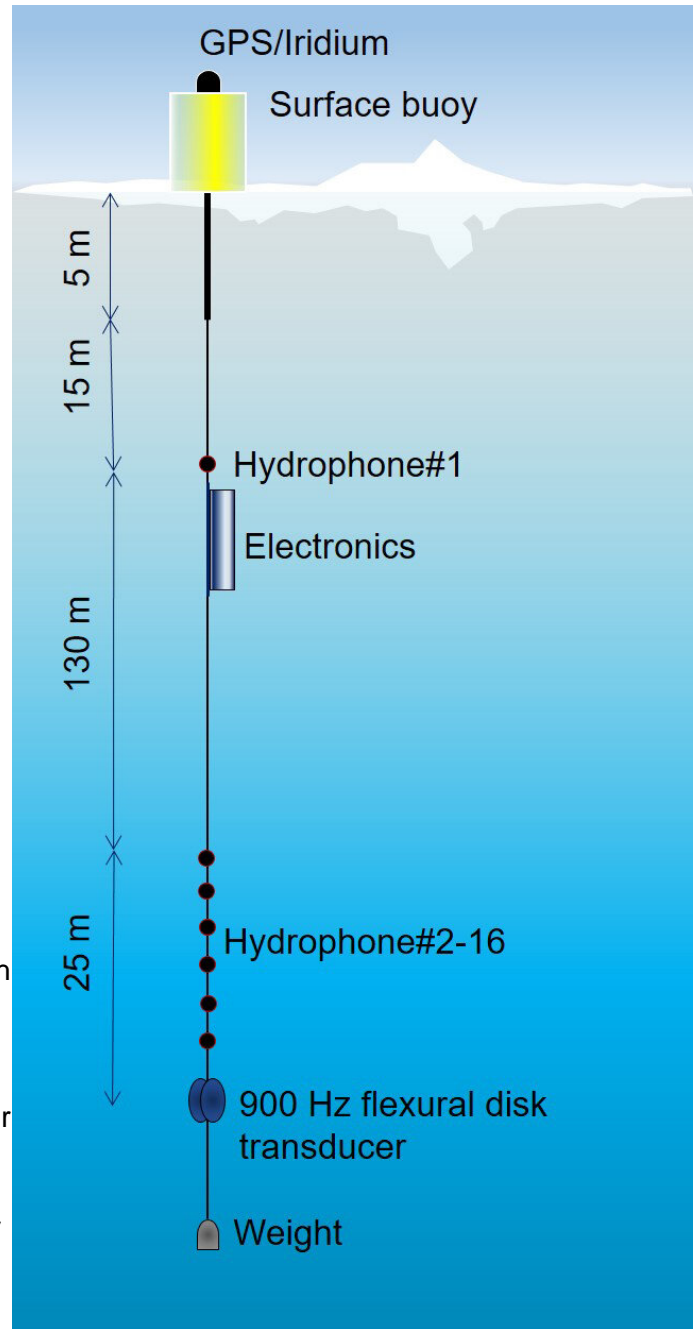
Components of a U.S. Naval Research Laboratory developed ce-tethered acoustic Buoy (ITAB). Credit: U.S. Naval Research Laboratory
