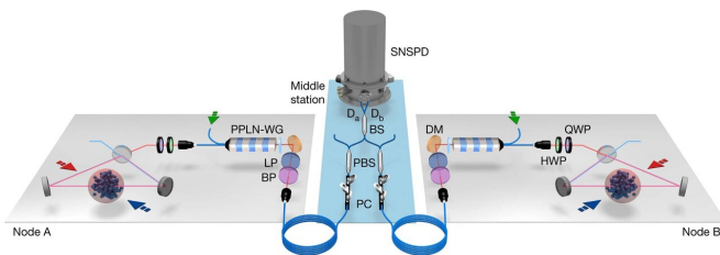
Schematic of the remote entanglement generation between atomic ensembles. Credit: Nature (2020). DOI: 10.1038/s41586-020-1976-7
