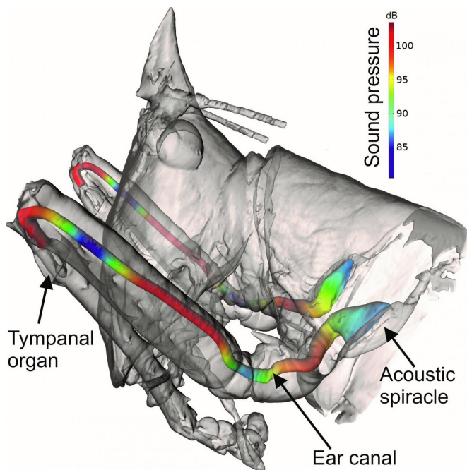
Pictured is a diagram of the bush-cricket Copiphora gorgonensis , which are found in the Colombian rainforest, showing how the sound pressure changes inside its 'ear canal'. Credit: Dr Thorin Jonsson
