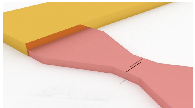
High temperature superconducting microbridge (pink) in gold contacts (yellow). Credit: M. Lyatti et al/Nature Communications
