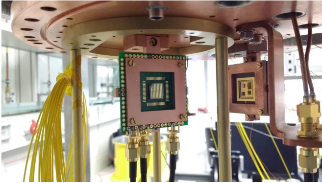
The measurement setup for the characterization of microbridges in a cryostat. Credit: Martin Wolff
