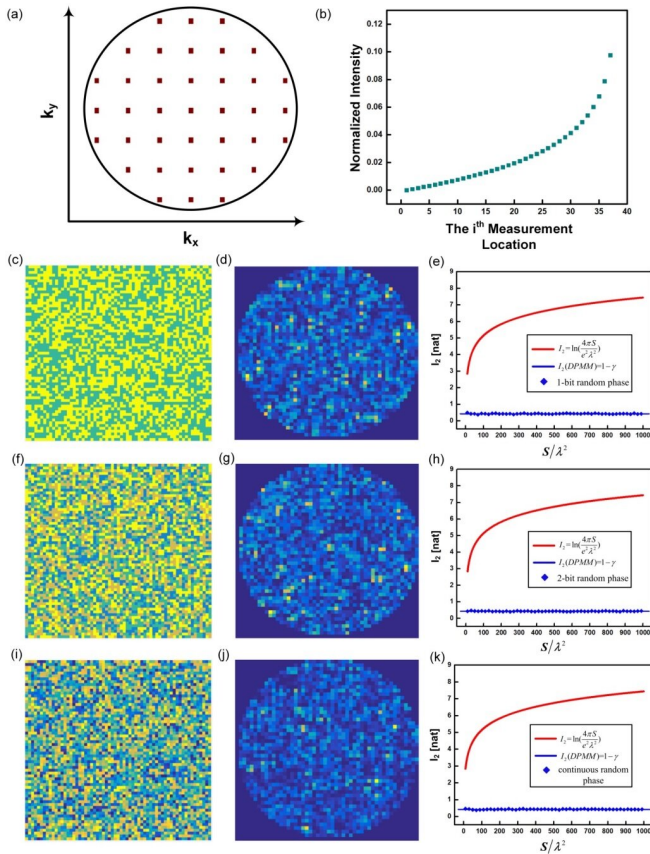
(a) A set of measurement locations in k -space. (b) Theoretical intensity distributions of the measurement points. (c, d) A sample of 1-bit disordered-phase pattern of the metasurface and the generated far-field intensity distribution. (e) Theoretical and calculated results of I_2 (information of the radiation pattern) with respect to different sizes and phase patterns of the metasurfaces. (f, g) A sample of 2-bit disordered-phase pattern of metasurface and the generated far-field intensity distribution. (h) Theoretical and calculated results of I_2 with respect to different sizes and phase patterns of metasurfaces. (i, j) A sample of continuous disordered-phase pattern of the metasurface and the generated far-field intensity distribution. (k) Theoretical and calculated results of I_2 with respect to different sizes and phase patterns of metasurfaces. Credit: ©Science China Press
