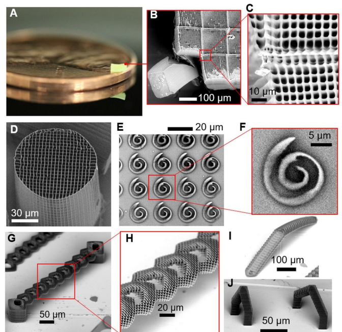
Fig. 1. Printing of complex 3D structures with submicron resolution via FP-TPL. (A to C) Millimeter-scale structure with submicrometer features supported on a U.S. penny
