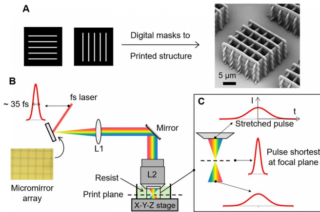
FP-TPL based on spatial and temporal focusing. Credit: CUHK
