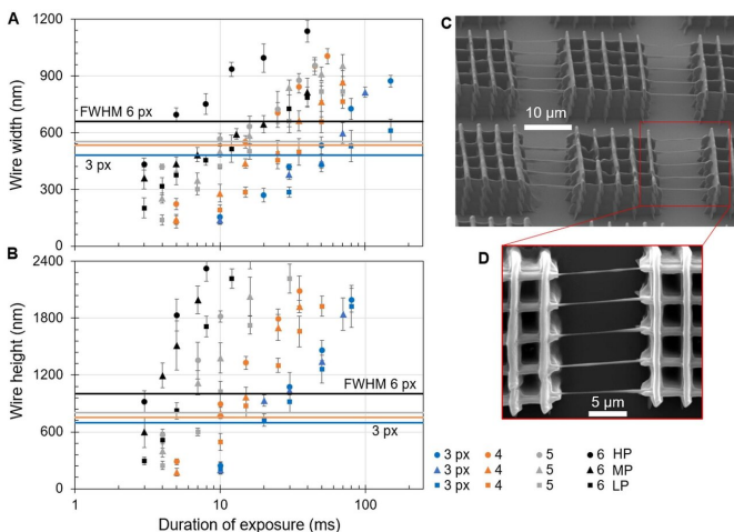
Fig. 2. Printed nanowires demonstrating nanoscale resolution of FP-TPL. (A) Width (along lateral direction) and (B) height (along axial direction) of suspended nanowires printed under different conditions. Width of lines in the projected DMD pattern was varied from 3 to 6 pixels with a fixed period of 30 pixels. Each pixel (px) maps to 151 nm in the projected image. Labels HP, MP, and LP refer to high (42 nW/px), medium (39 nW/px), and low (35 nW/px) power levels, respectively. All markers of a specific shape represent data points generated at the same power level, and all markers of a specific colour represent the same line width. Printing was performed with a femtosecond laser that had a center wavelength of 800 nm and a nominal pulse width of 35 fs and with a 60 × 1.25 numerical aperture objective lens. (C and D) Scanning electron microscope images of the suspended
