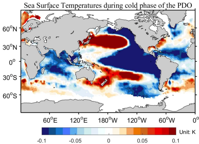
Sea surface temperatures during cold phase of PDO. Credit: CSHOR
