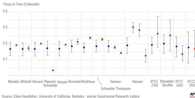
Source: Zeke Hausfather, University of California, Berkeley; journal Geophysical Research Letters
