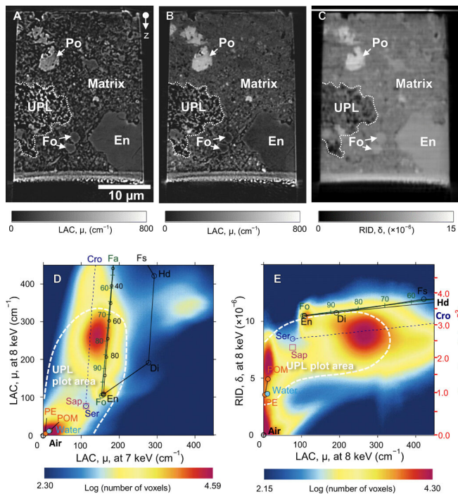
XCT slice images of equant samples of the Acfer 094 matrix and their 2D histograms of LAC and RID values at 7 and 8 keV. Absorption XCT images at 7 keV (A) and 8 keV (B), as well as a phase XCT image at 8 keV (C), indicate an UPL embedded in the matrix. 2D histograms of LAC values at 7 and 8 keV (D) and LAC and RID values at 8 keV (E) of the matrix show peaks around the air, resin [polyacetal (POM)], forsterite (Fo), enstatite (En), and serpentine/saponite (Serp/Sap)–cronstedtite (Cro). Those plots of UPL have peaks in the areas surrounded by white dashed lines in (D) and (E). The density scale corresponding to the RID values is shown in (E). Fa, fayalite; Di, diopside; Hd, hedenbergite; Fs, ferrosilite; Po, pyrrhotite; PE, polyethylene. Credit: Science Advances (2019). DOI: 10.1126/sciadv.aax5078
