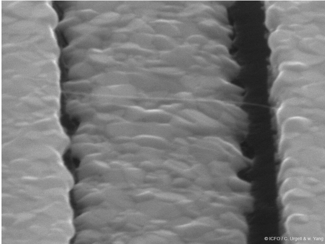
Carbon nanotube resonator clamped between two electrodes. Credit: © ICFO/ C. Urgell & W. Yang
