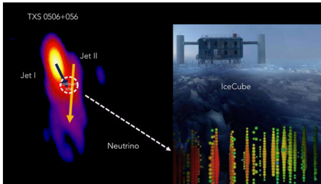
TXS 0506+056. The neutrino event IceCube 170922A appears to originate in the interaction zone of the two jets. Credit: IceCube Collaboration, MOJAVE, S. Britzen, & M. Zaja?ek
